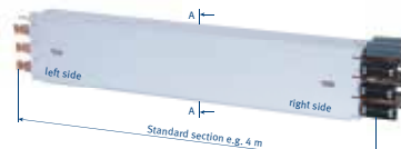
Type MKHF with plug in joints, factory assembled
