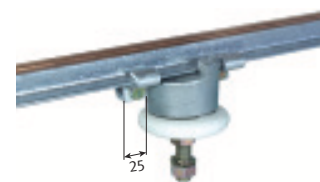
Illustration shows an insulator with 2 locating clamps (fix point)
