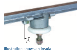
Illustration shows an insulator with 2 locating clamps
